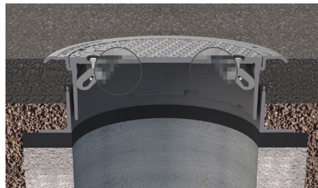
The SELFLEVEL® access assembly requires two VERSACAM security locks and security bolts.
