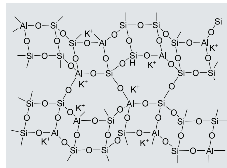
An example theoretical chemical structure of an Aluminosilicate geopolymer
